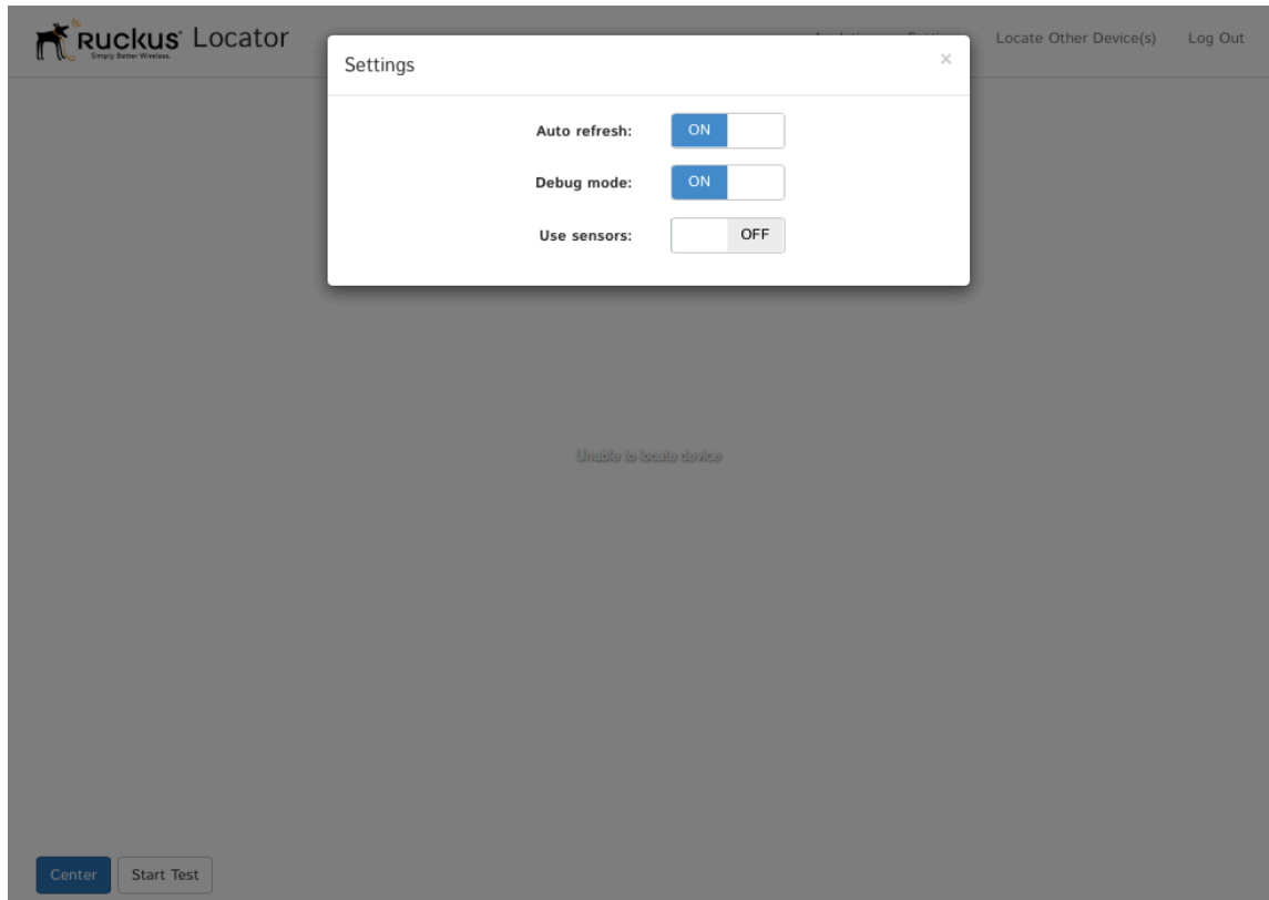
FIGURE 126 Locator Settings
