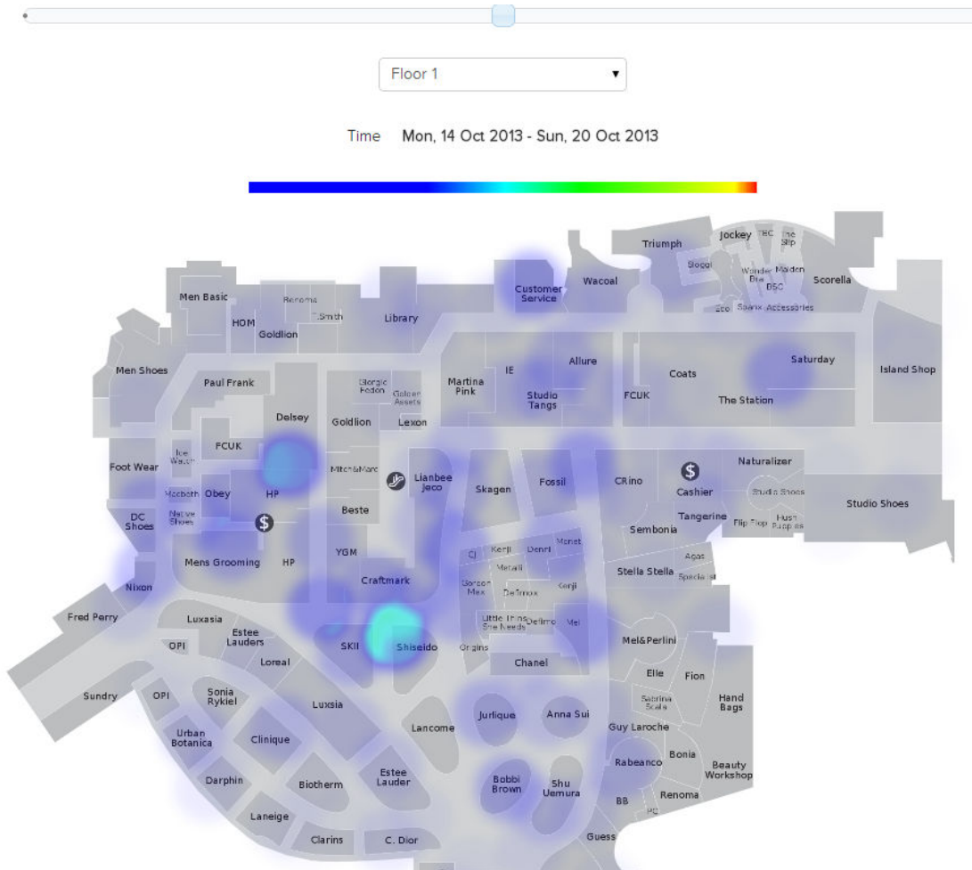
FIGURE 117 Heatmap
