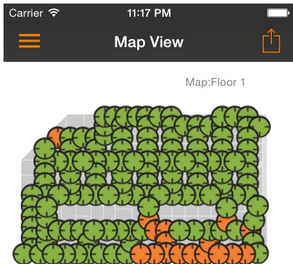
FIGURE 54 Start Calibration
