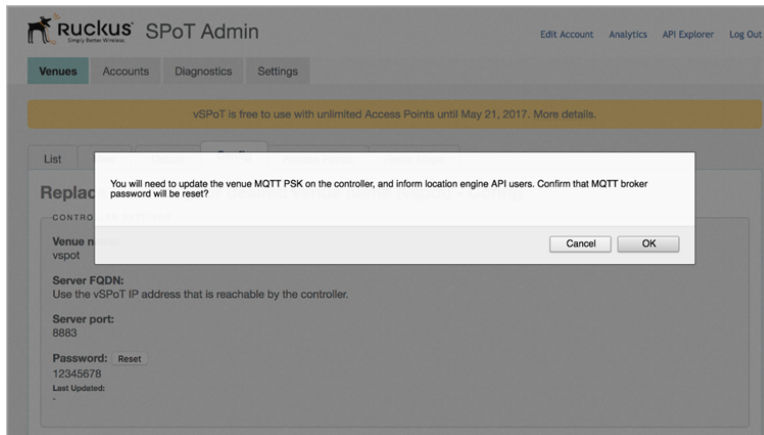
FIGURE 102 Reset password
