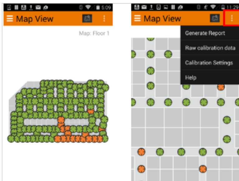
FIGURE 36 Options
