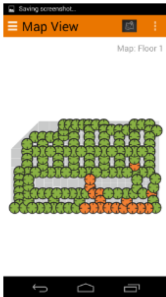
FIGURE 29 CPs marked
